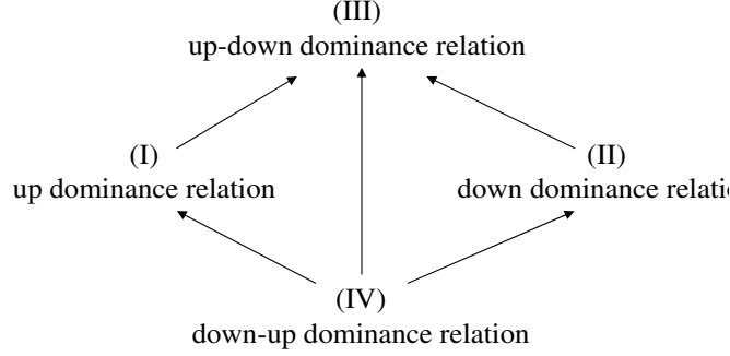
Figure 3.1 Superset-subset relationship among the four types of dominance relations
