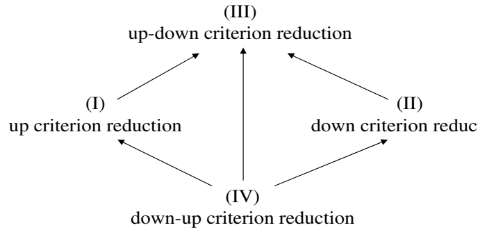
Figure 6.1 Superset-subset relationship among the four types of criterion reductions
