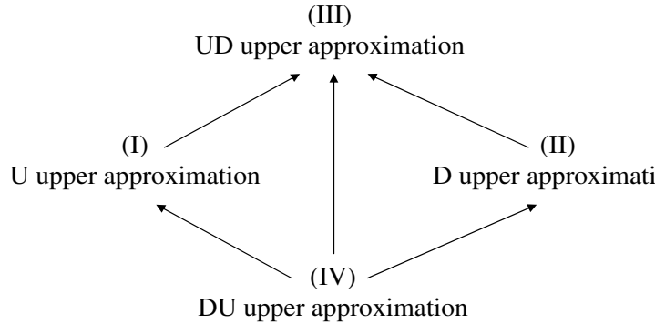
Figure 4.2 Inclusion relationship among the four types of upper approximations
