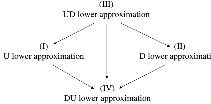
Figure 4.1 Inclusion relationship among the four types of lower approximations
